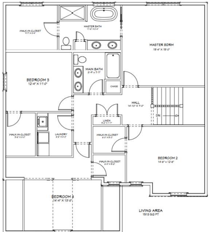
SECOND FLOOR
